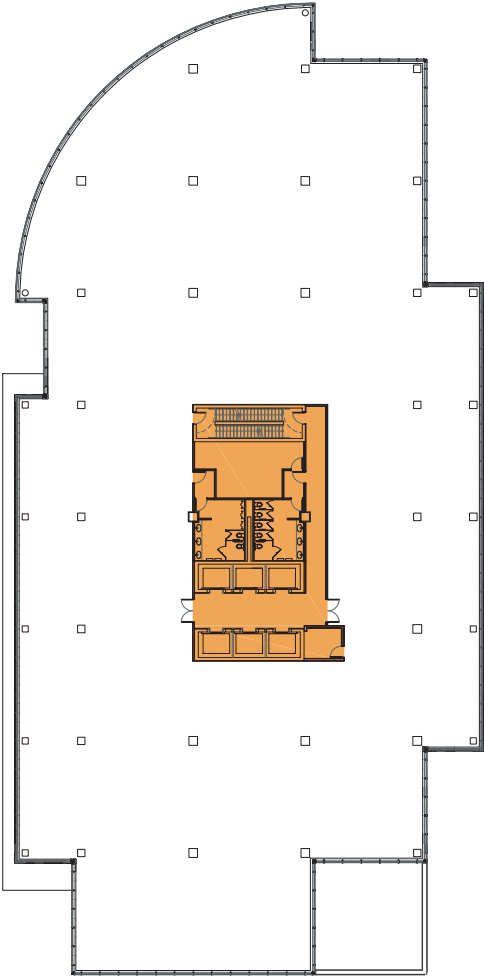
PHASE II (BUILDING I) TYPICAL SINGLE-TENANT 6th-8th FLOORS
