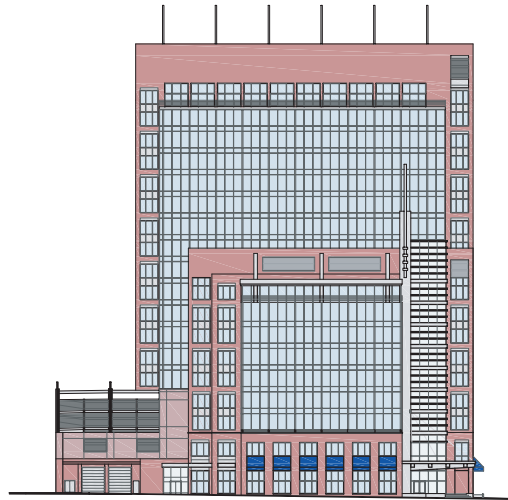
PHASE II SOUTH ELEVATION
