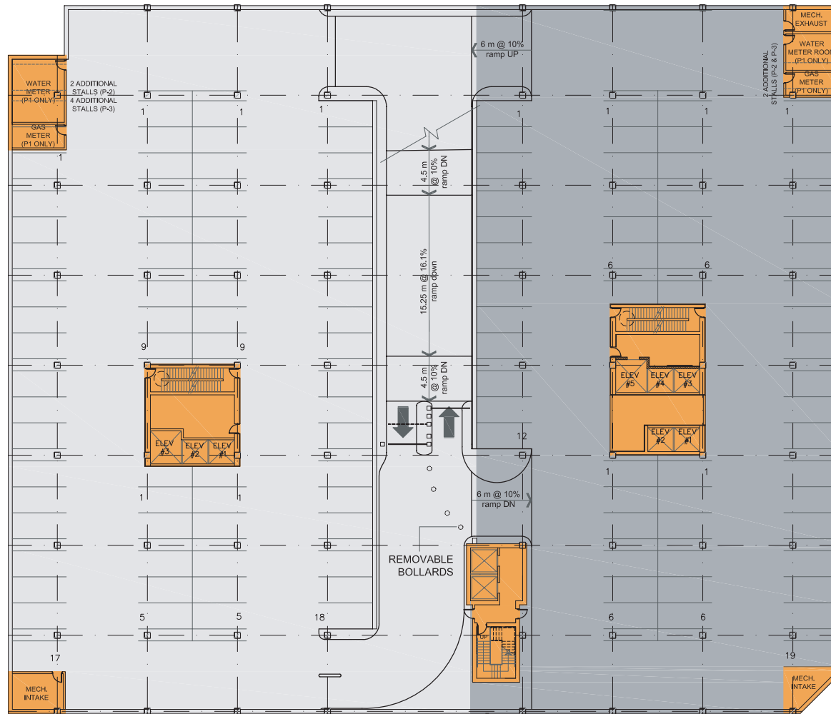
PHASE II UNDERGROUND PARKING B1, B2, B3
